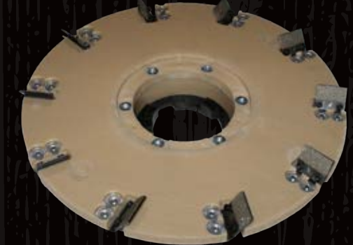
Mastic Removal Tool 56383926 use with Epoch HD, RS-16DC, Sander 1600
